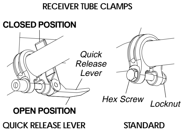
FIGURE 6 - OPENING/CLOSING CLAMPS
